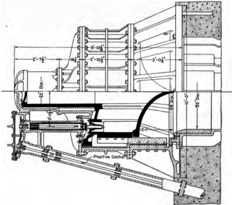
FIG. 42.—58-inch balanced valve with positive control for reservoir outlet from plans by U. S. Reclamation Service.
